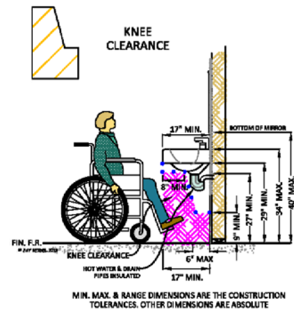
SIDE ELEVATION - KNEE CLEARANCE AND SINK MOUNTING DIMENSIONS
