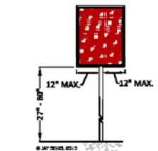
POST MOUNTED PROTRUDING OBJECTS 11B-307.3 (a)
